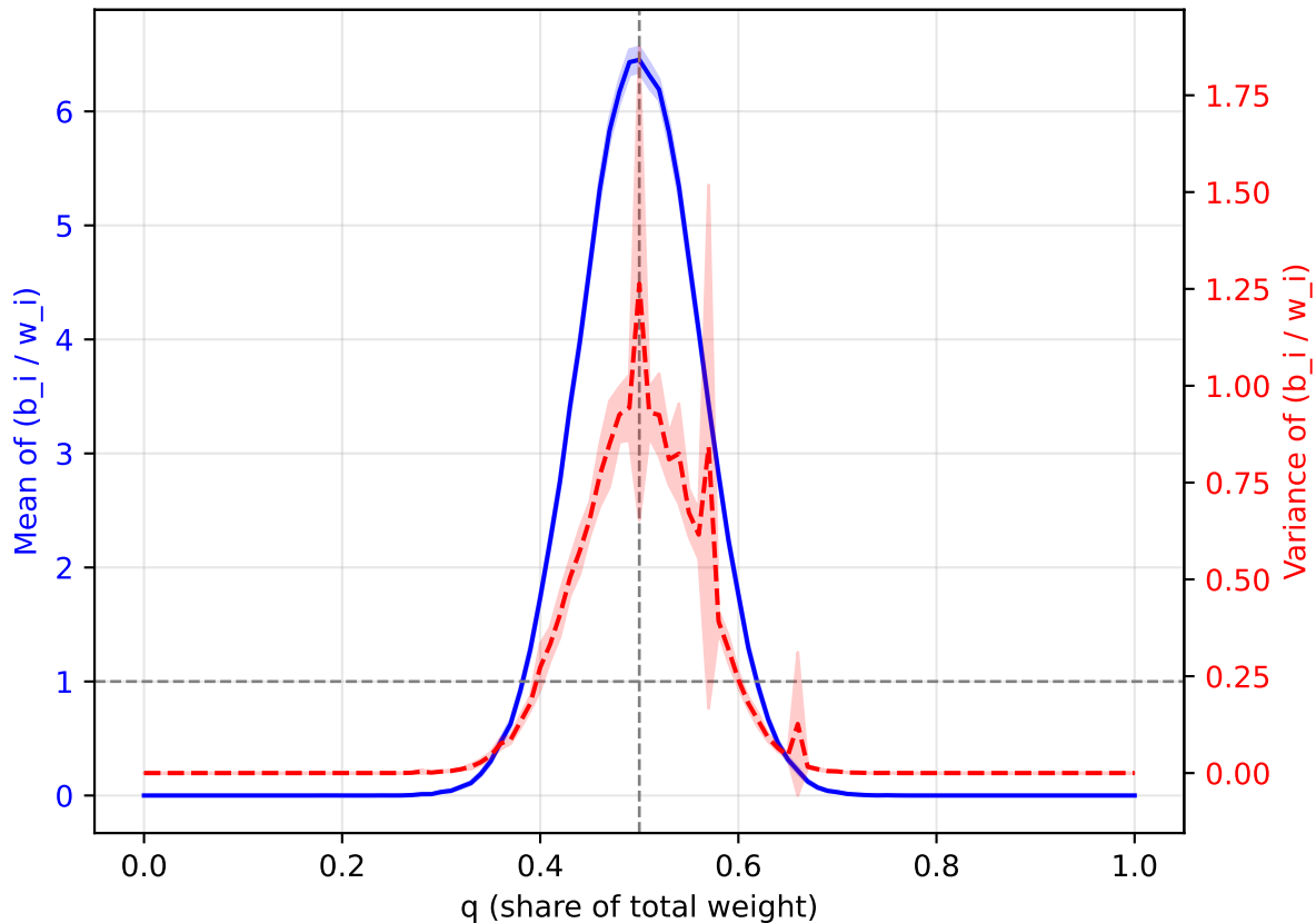
Gamma( \alpha=2.0 , \theta=2.0 ) — mean-of-means & mean-of-vars
