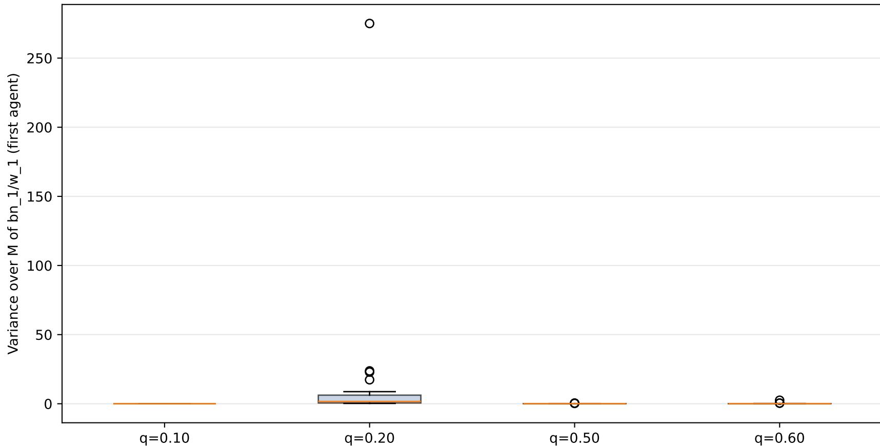
Gamma( \alpha=0.5 , \theta=1.0 ) — First agent variance across 20 repeats at multiple quotas
