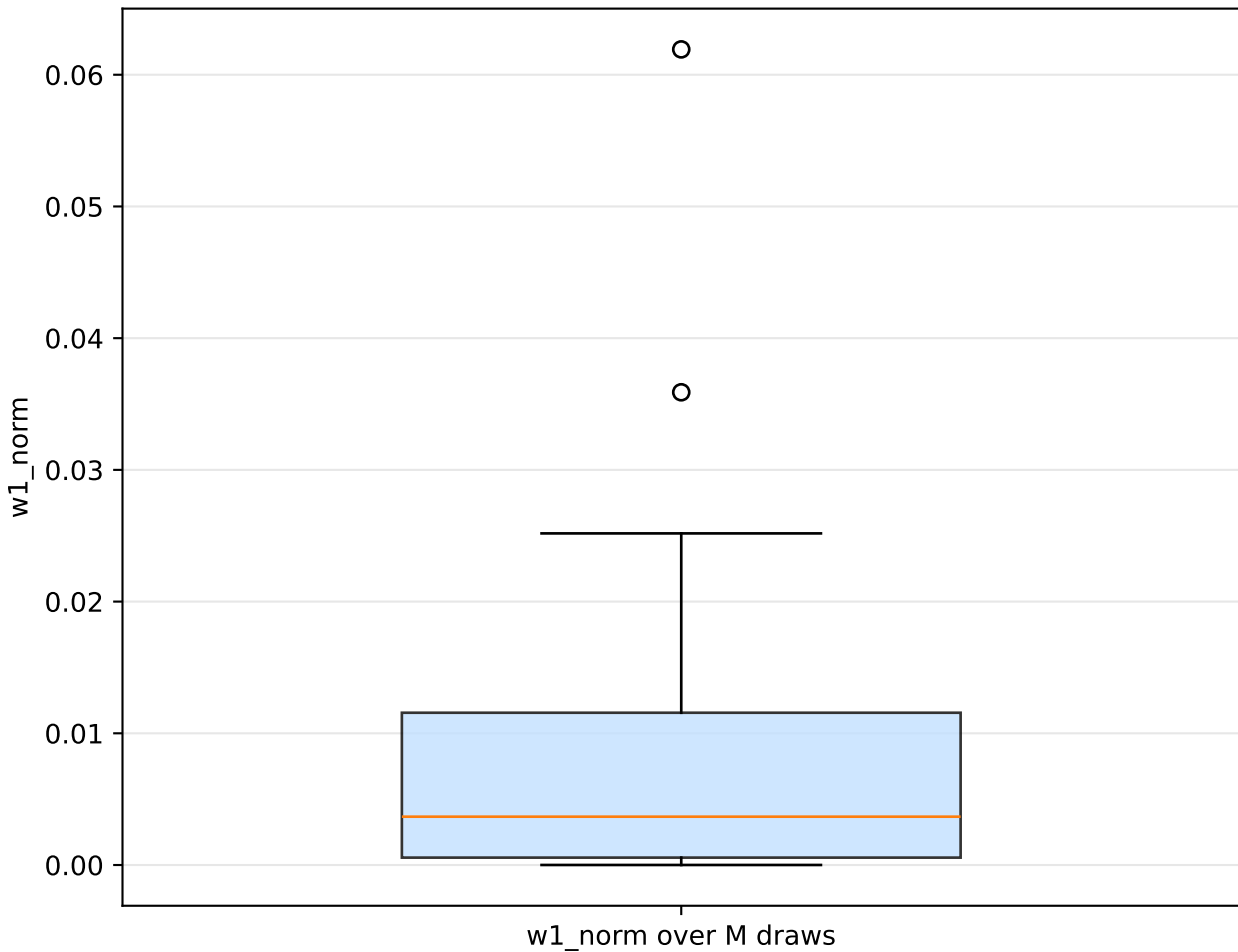
Gamma( \alpha=0.5 , \theta=1.0 ) — First agent normalized weight distribution
