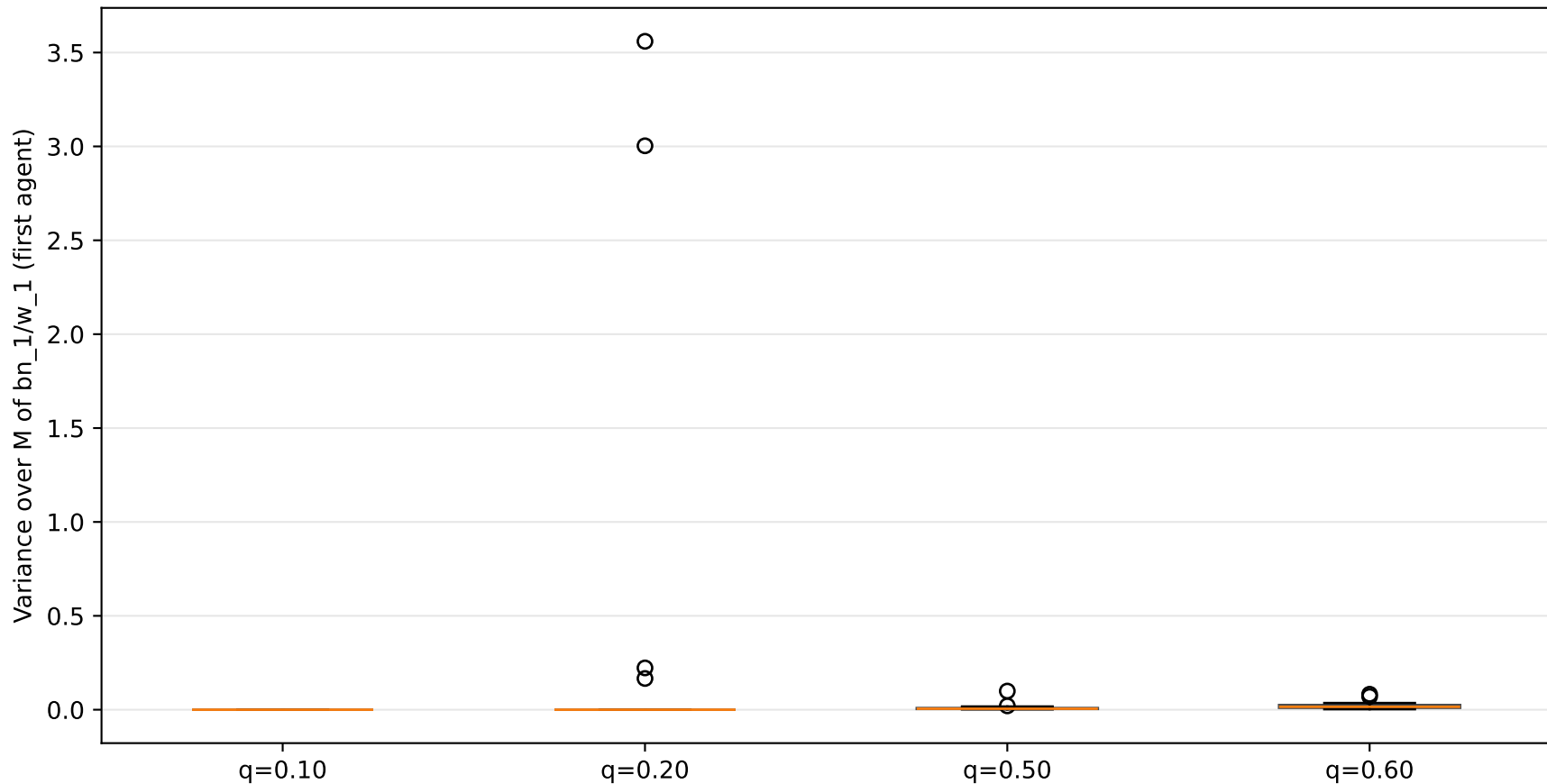
Gamma( \alpha=1.0 , \theta=0.5 ) — First agent variance across 20 repeats at multiple quotas
