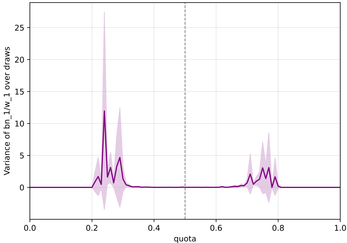
Gamma( \alpha=1.0 , \theta=0.5 ) — First agent ratio variance
