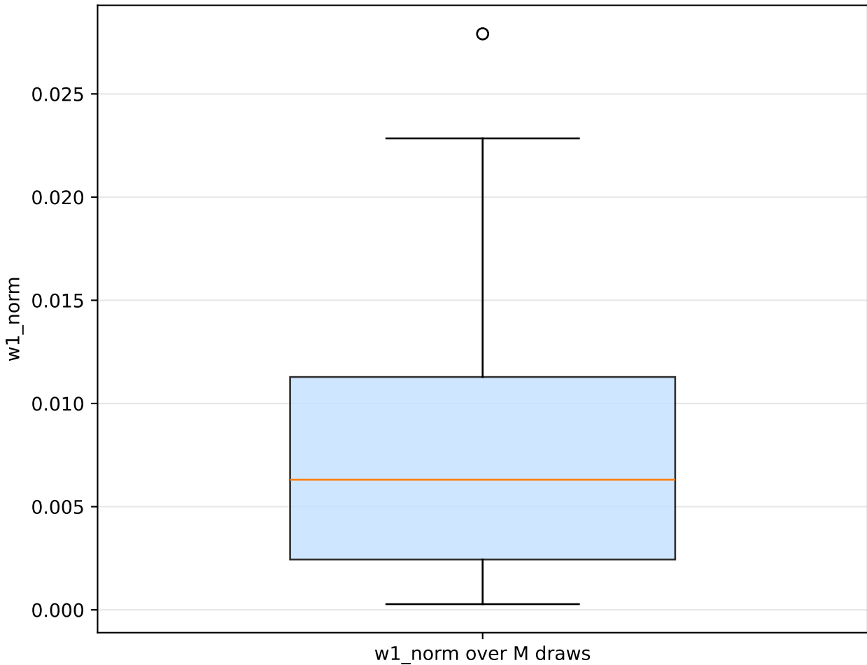
Gamma( \alpha=1.0 , \theta=0.5 ) — First agent normalized weight distribution
