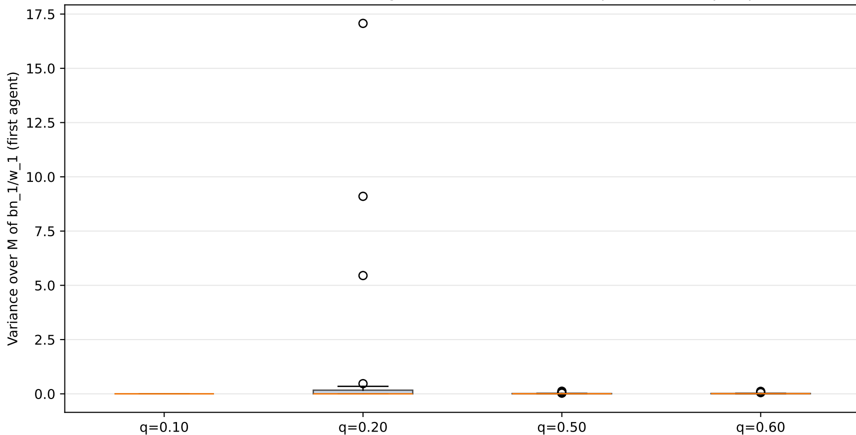
Gamma( \alpha=1.0 , \theta=1.0 ) — First agent variance across 20 repeats at multiple quotas
