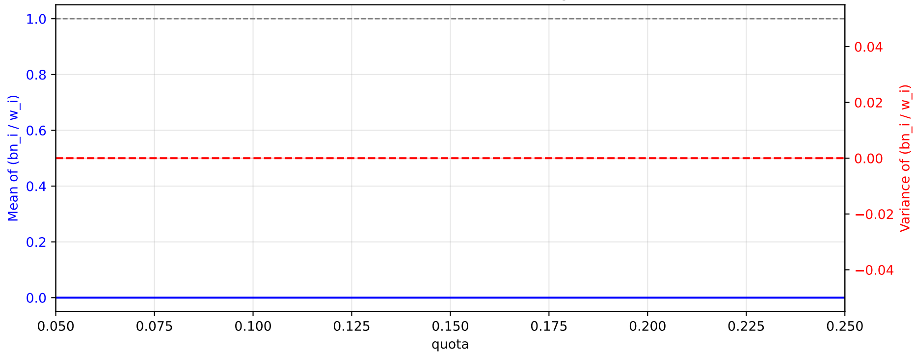
Gamma( \alpha=0.5 , \theta=2.0 ) — ratios and weight variance
