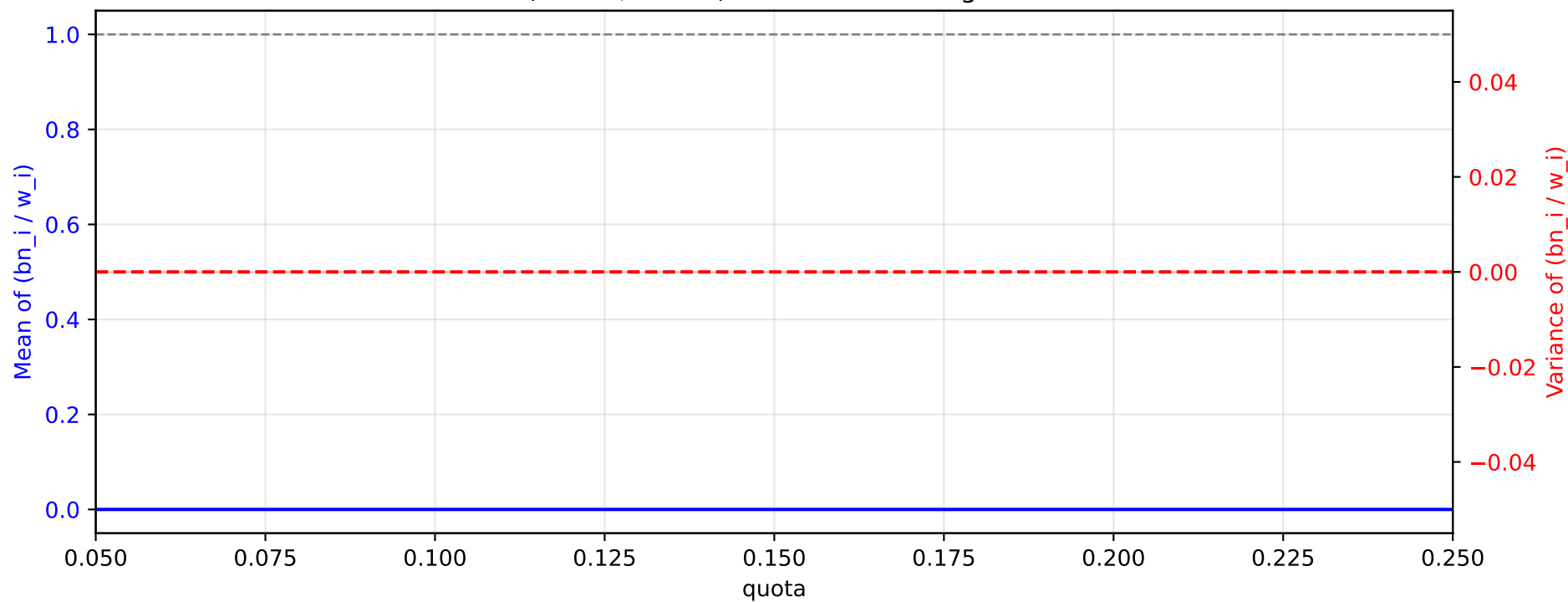
Gamma( \alpha=1.0 , \theta=0.5 ) — ratios and weight variance
