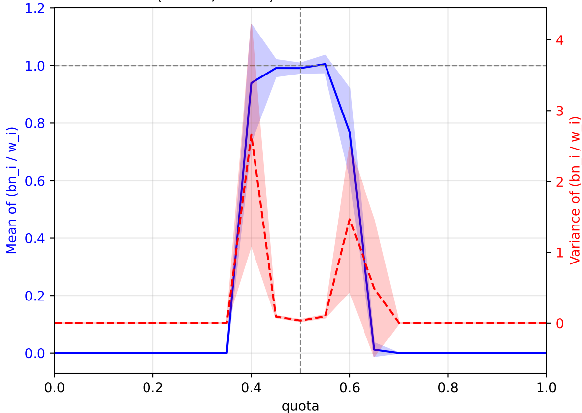
Gamma( \alpha=1.0 , \theta=0.5 ) — normalized Banzhaf ratios
