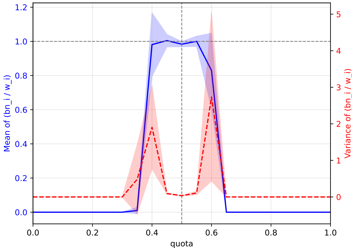
Gamma( \alpha=1.0 , \theta=1.0 ) — normalized Banzhaf ratios
