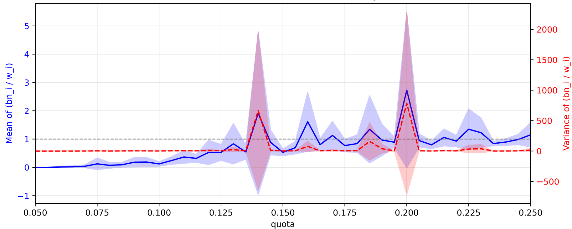
Gamma( \alpha=0.24 , \theta=330235.0 ) — ratios and weight variance
