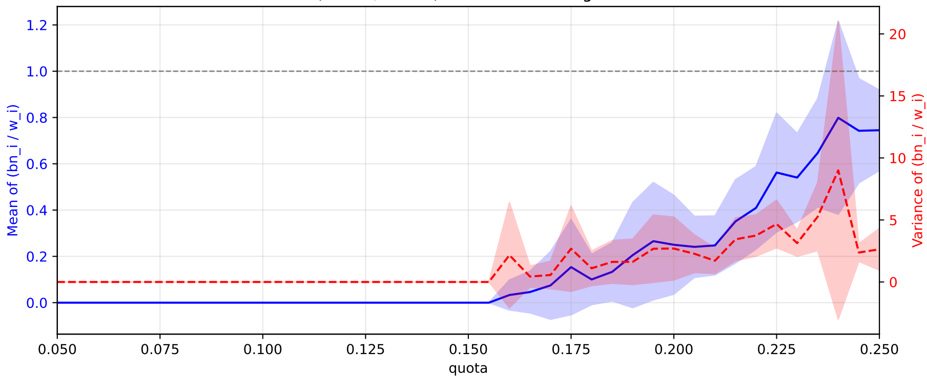
Gamma( \alpha=1.0 , \theta=1.0 ) — ratios and weight variance
