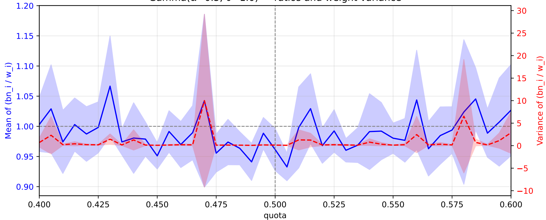
Gamma( \alpha=0.5 , \theta=1.0 ) — ratios and weight variance
