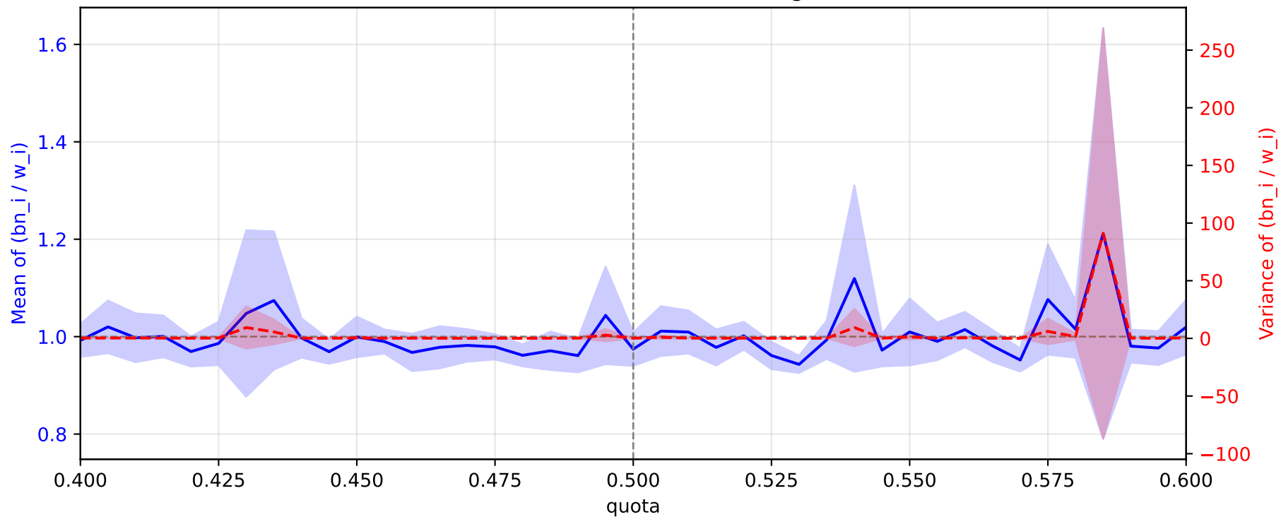
Gamma( \alpha=0.5 , \theta=2.0 ) — ratios and weight variance
