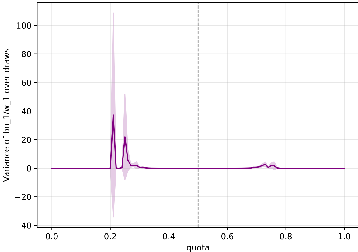
Gamma( \alpha=2.0 , \theta=1.0 ) — First agent ratio variance
