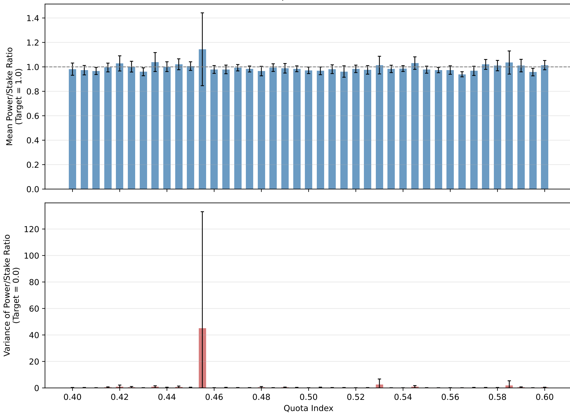
Fairness Summary by Quota (n=100) Gamma(Shape \alpha=0.5 , Scale \theta=1.0 )
