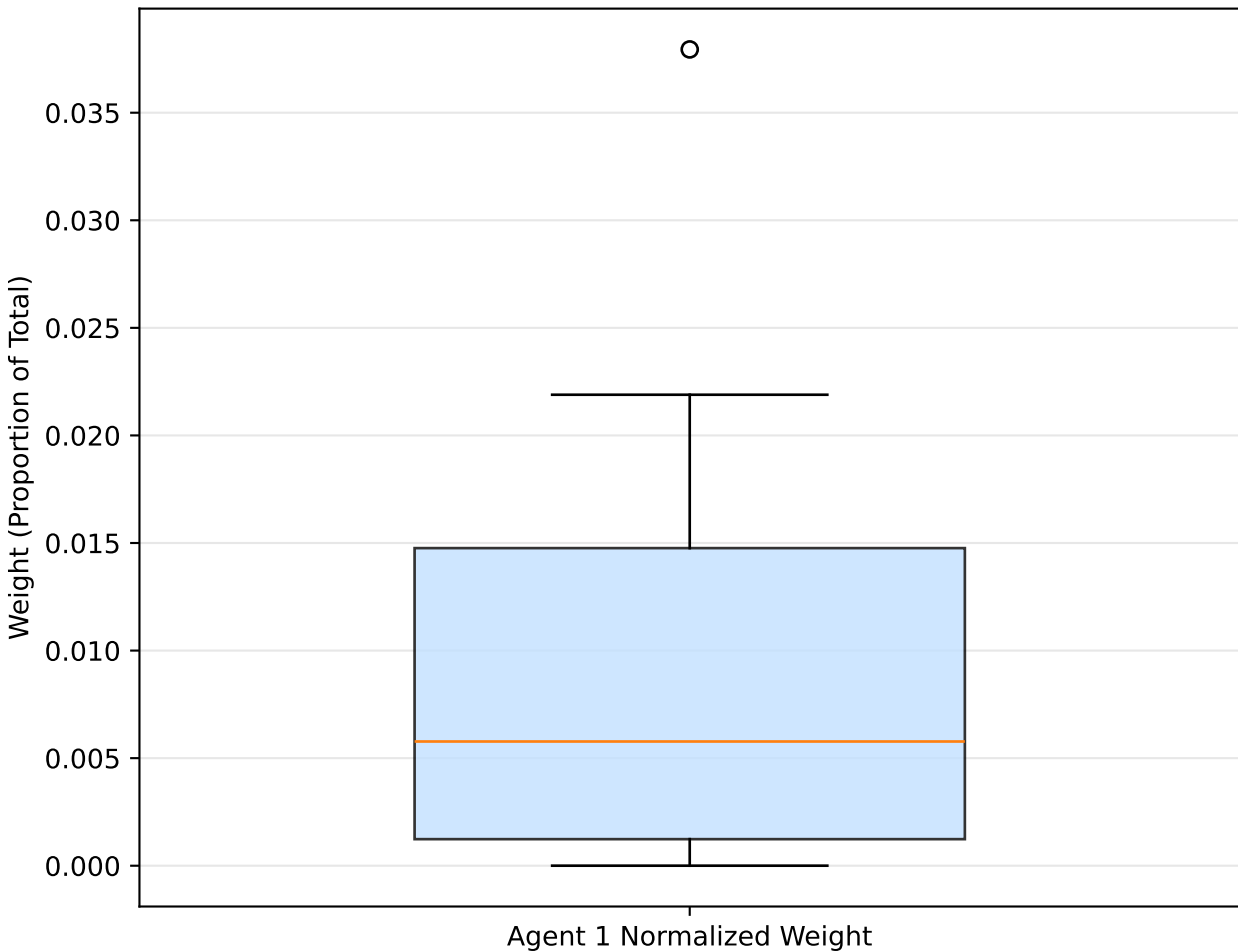
Agent 1 Weight Distribution (Gamma \alpha=0.5 , \theta=0.5 )
