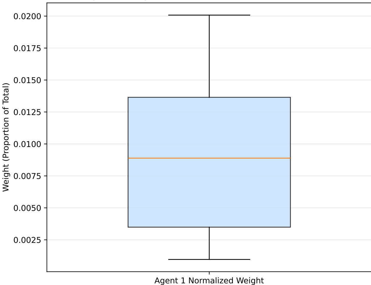
Agent 1 Weight Distribution (Gamma \alpha=1.0 , \theta=0.5 )
