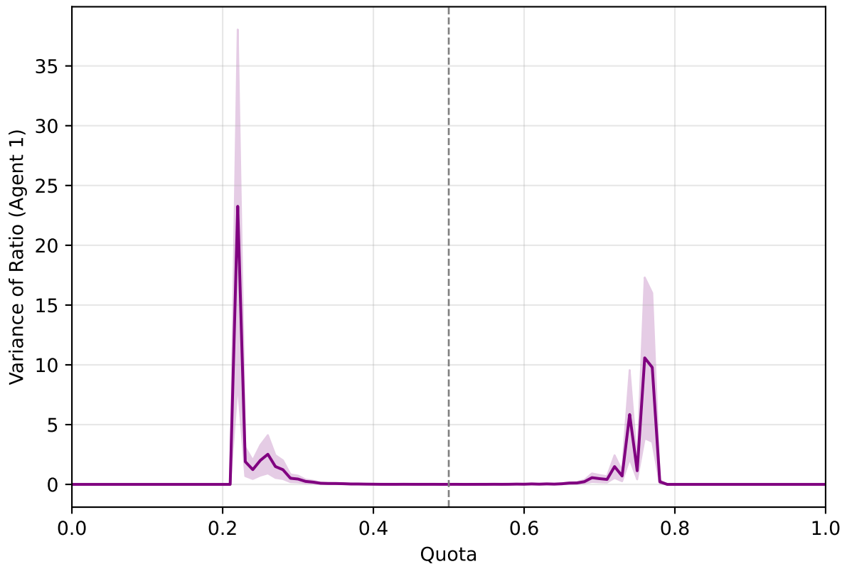
Stability Analysis: Agent 1 Ratio Variance Gamma( \alpha=1.0 , \theta=1.0 )
