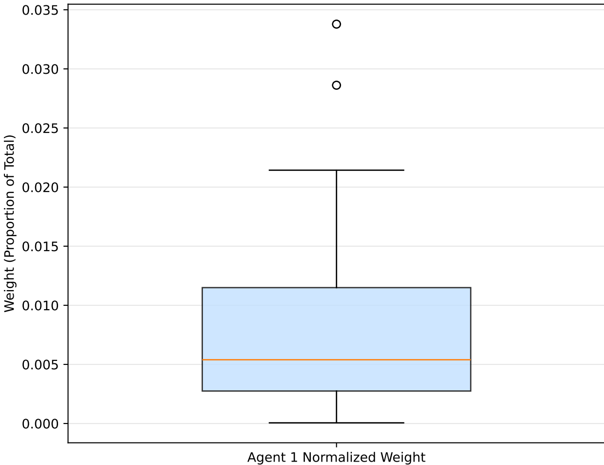
Agent 1 Weight Distribution (Gamma \alpha=1.0 , \theta=1.0 )
