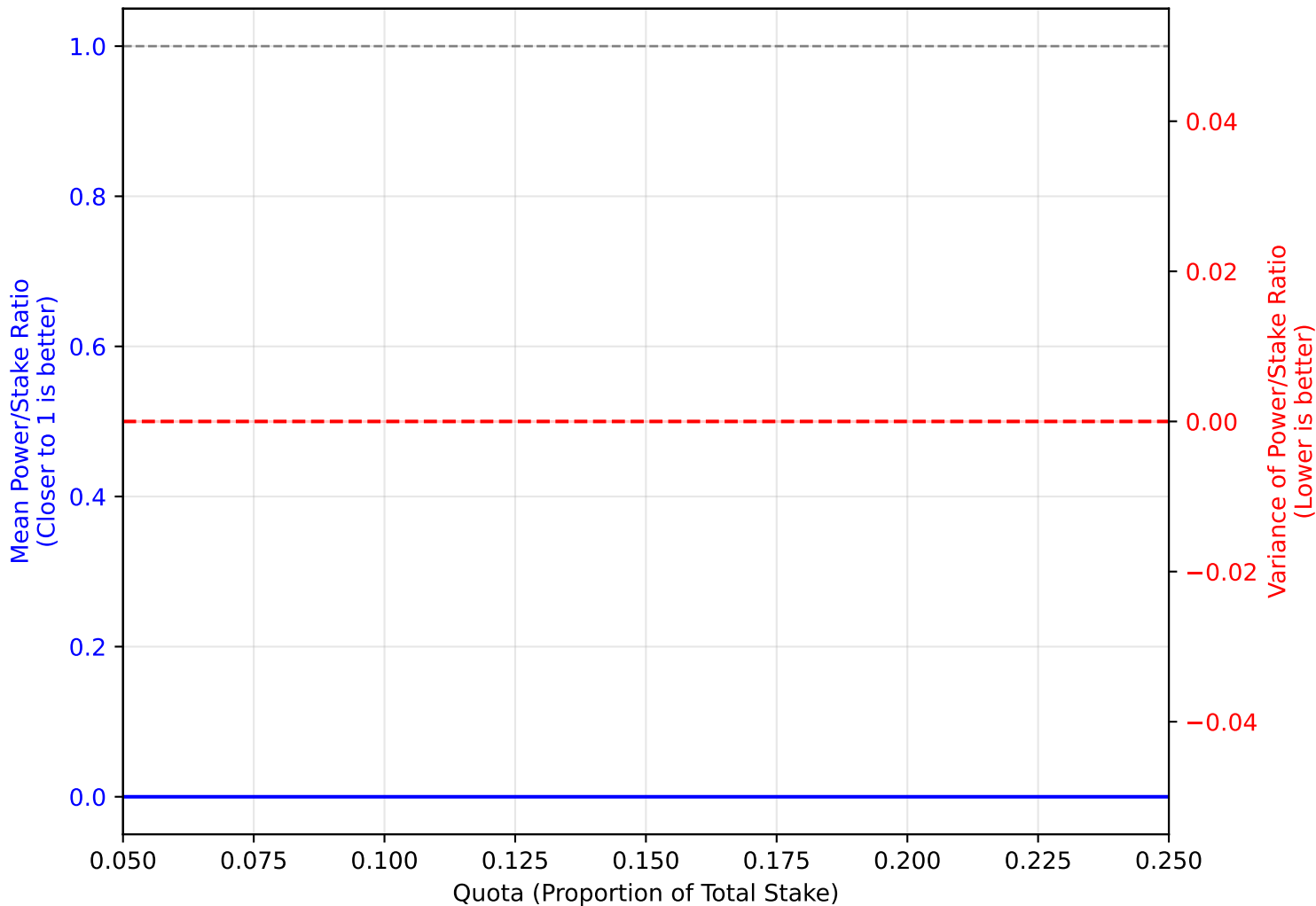
Fairness Analysis: Power vs. Stake Gamma Dist (Shape \alpha=1.0 , Scale \theta=1.0 , n=1000 )
