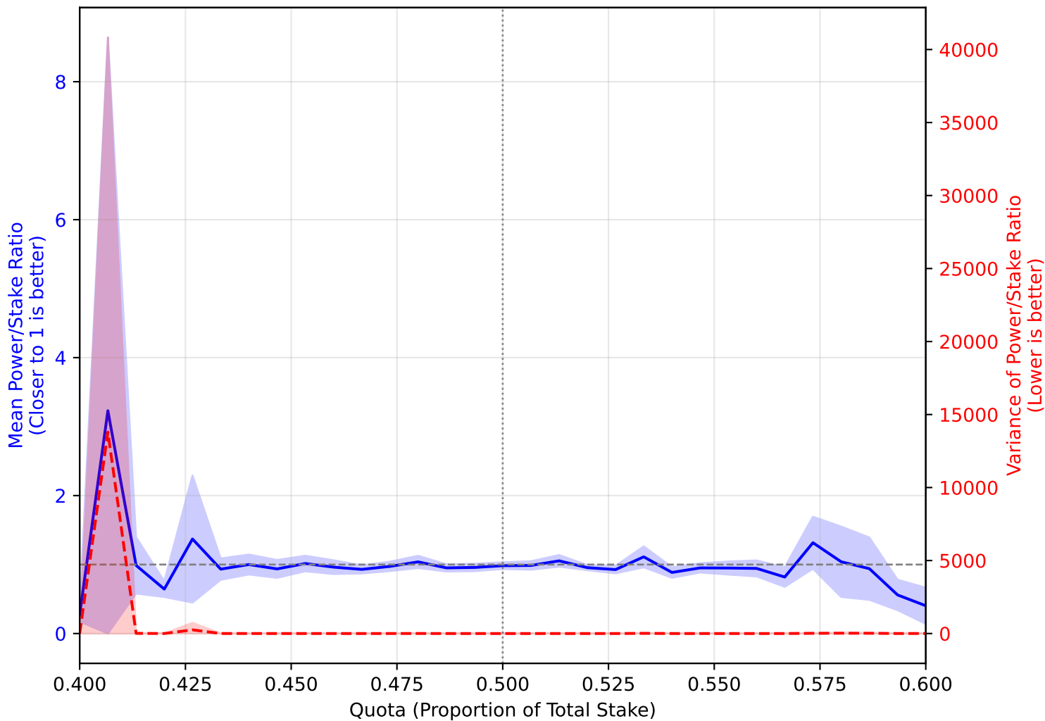
Fairness Analysis: Power vs. Stake Gamma Dist (Shape \alpha=0.5 , Scale \theta=2.0 , n=1000 )
