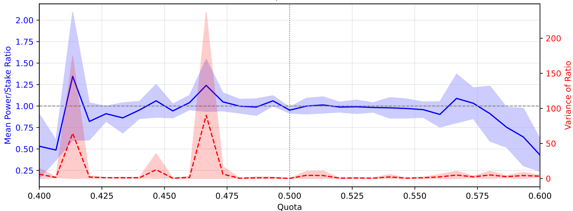
Fairness Metrics vs. Quota (n=1000) Gamma Dist (Shape \alpha=0.5 , Scale \theta=2.0 )
