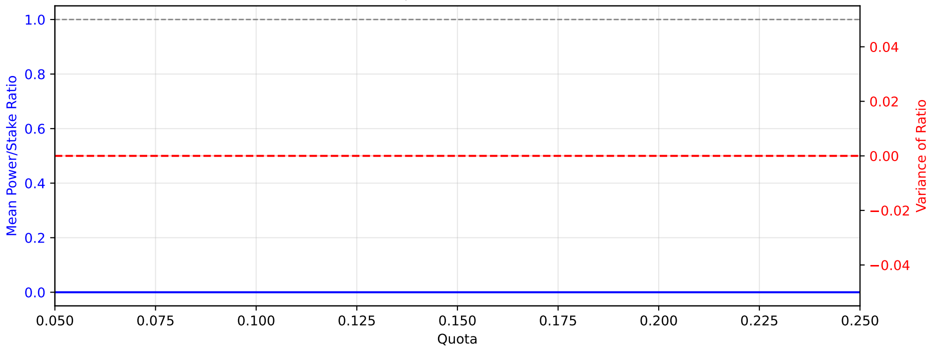
Fairness Metrics vs. Quota (n=500) Gamma Dist (Shape \alpha=0.24 , Scale \theta=330235.0 )
