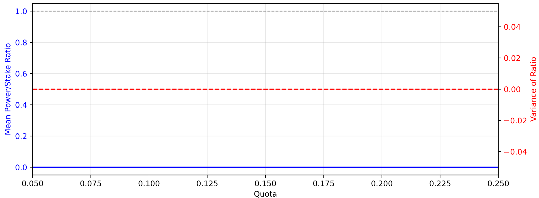
Fairness Metrics vs. Quota (n=500) Gamma Dist (Shape \alpha=0.5 , Scale \theta=0.5 )
