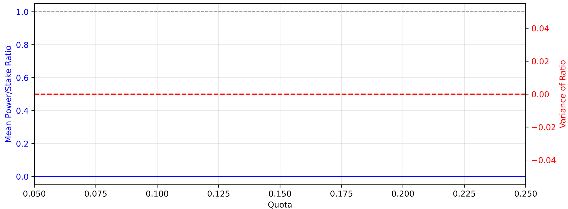
Fairness Metrics vs. Quota (n=500) Gamma Dist (Shape \alpha=0.5 , Scale \theta=1.0 )
