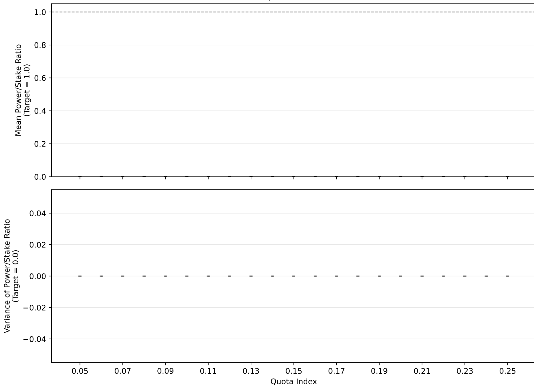
Fairness Summary by Quota (n=500) Gamma(Shape \alpha=1.0 , Scale \theta=0.5 )
