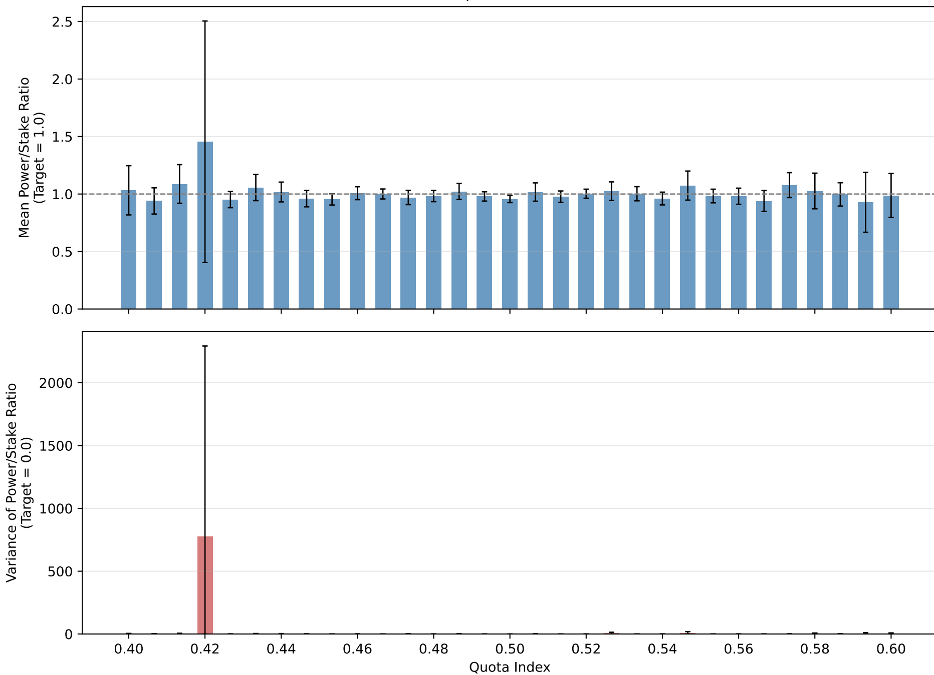
Fairness Summary by Quota (n=500) Gamma(Shape \alpha=0.5 , Scale \theta=2.0 )
