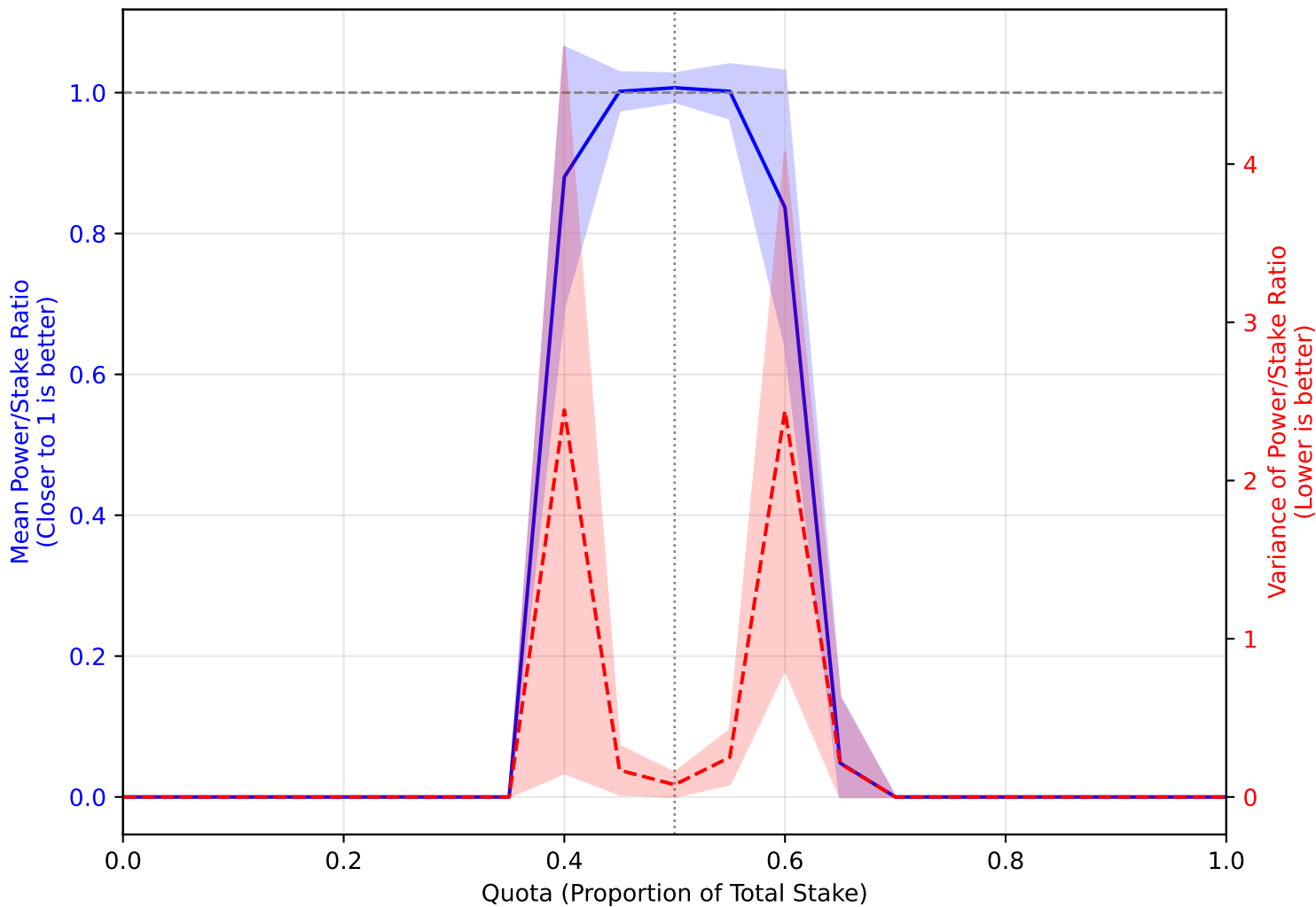
Fairness Analysis: Power vs. Stake Gamma Dist (Shape \alpha=1.0 , Scale \theta=1.0 , n=500 )
