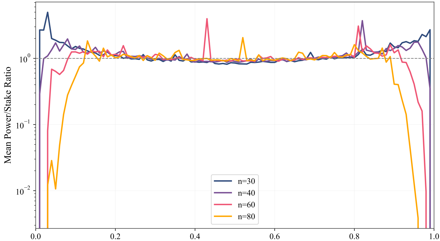
Mean Ratio vs Quota Gamma( \alpha=0.273568 , \theta=1301506.236646 )
