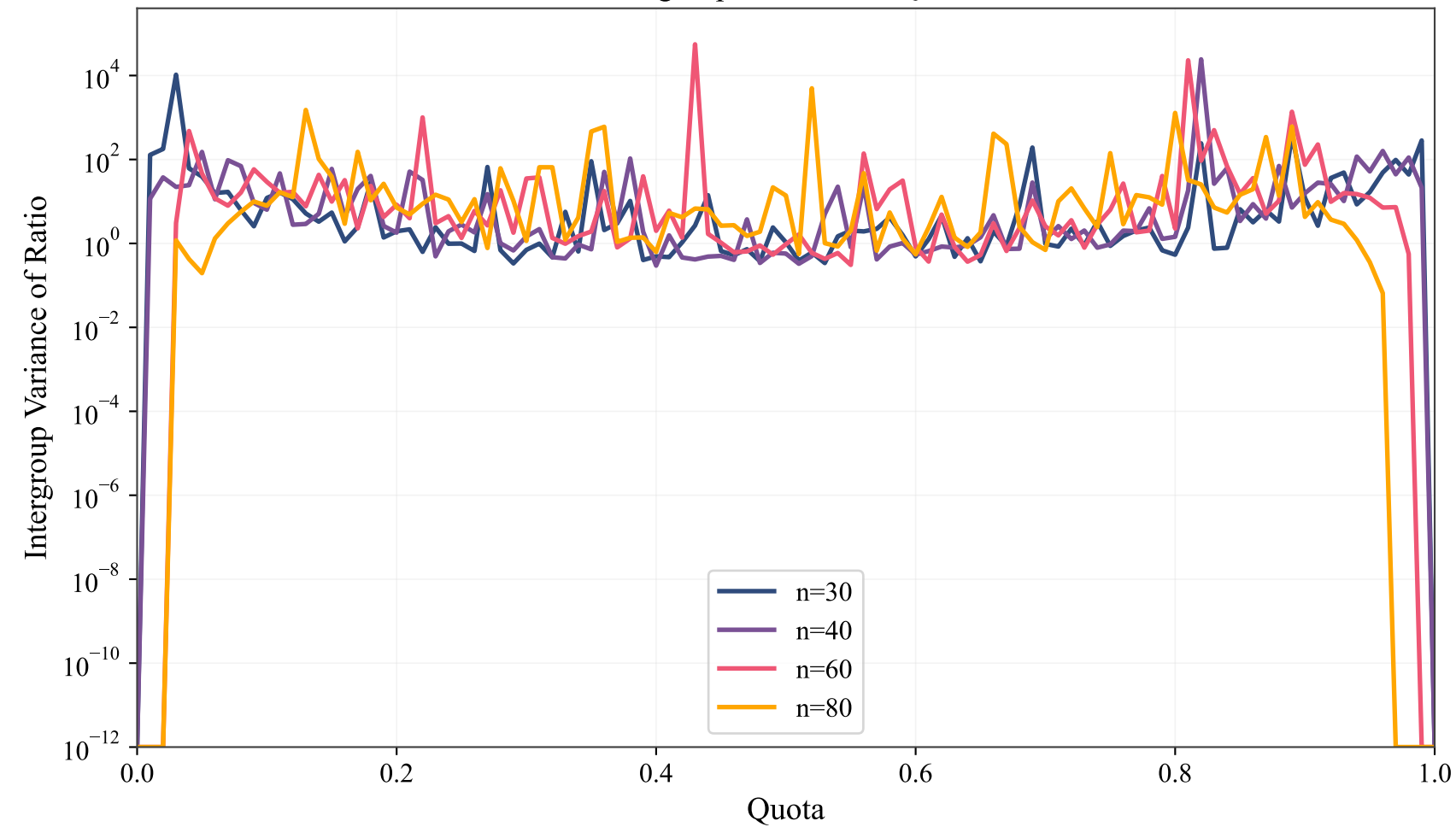
Intergroup Variance vs Quota
