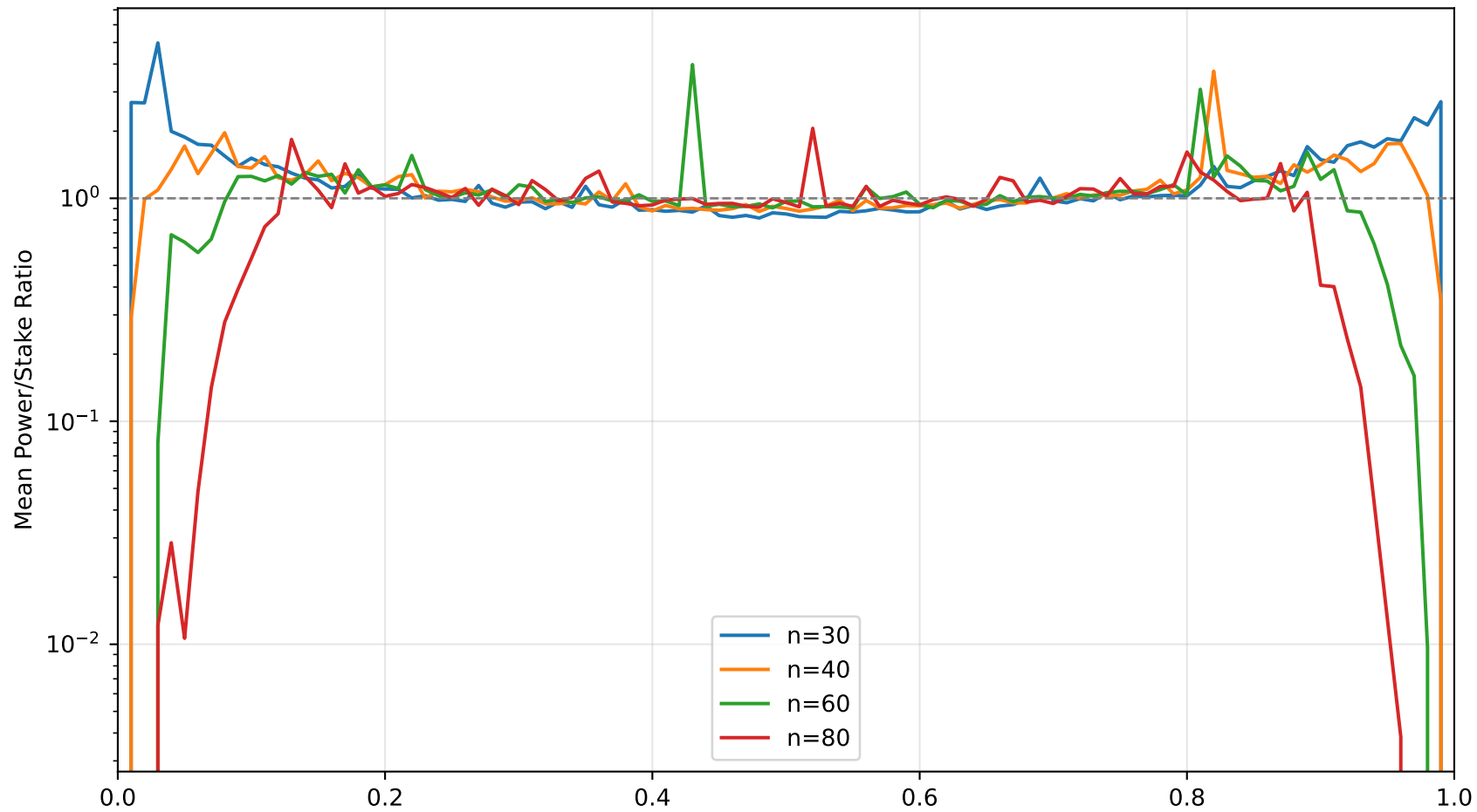
Mean Ratio vs Quota \text{Gamma}(\alpha=0.273568, \theta=1301506.236646)
