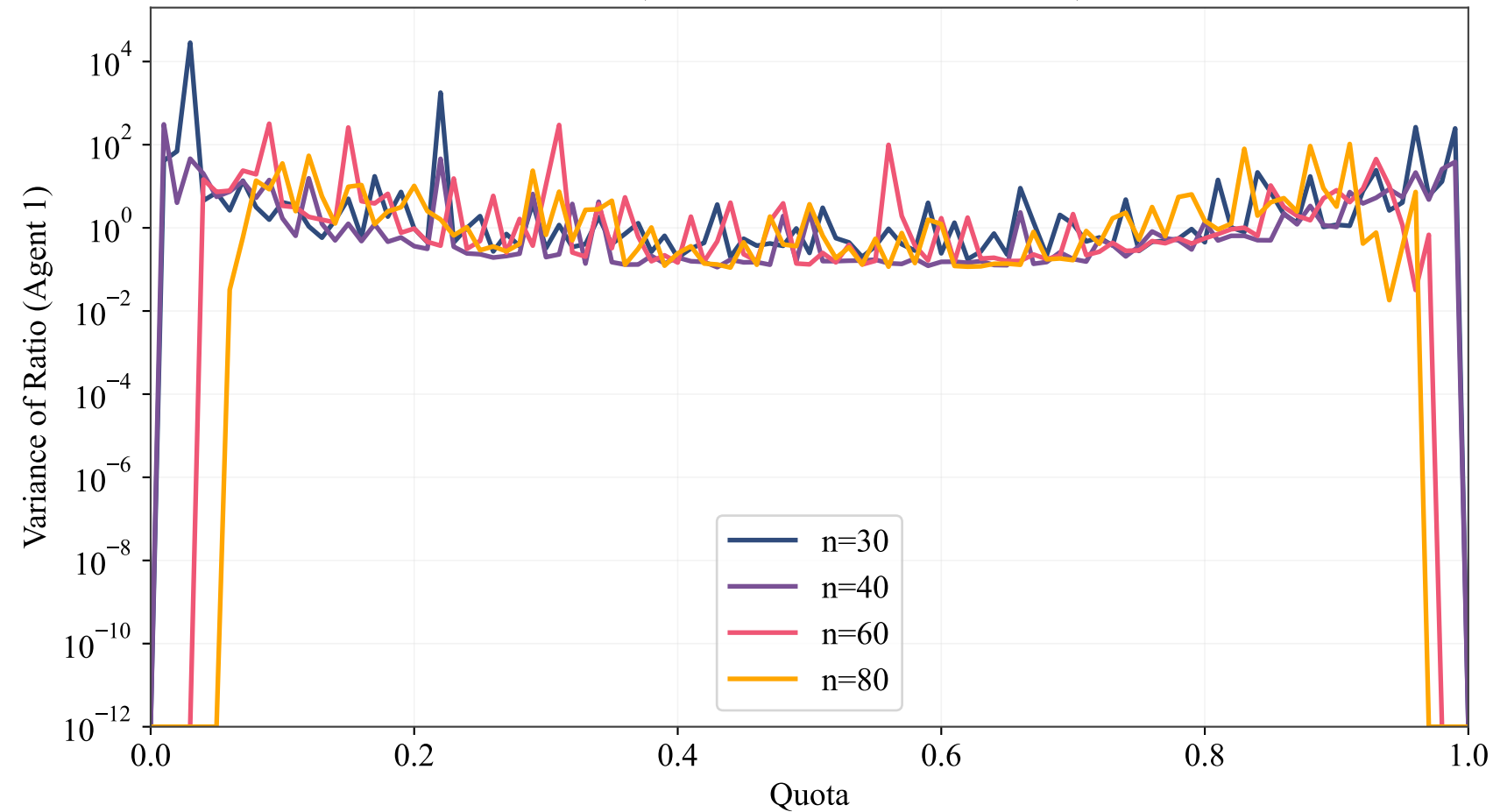
Agent 1 Ratio Variance vs Quota Gamma( \alpha=0.273568 , \theta=1301506.236646 )
