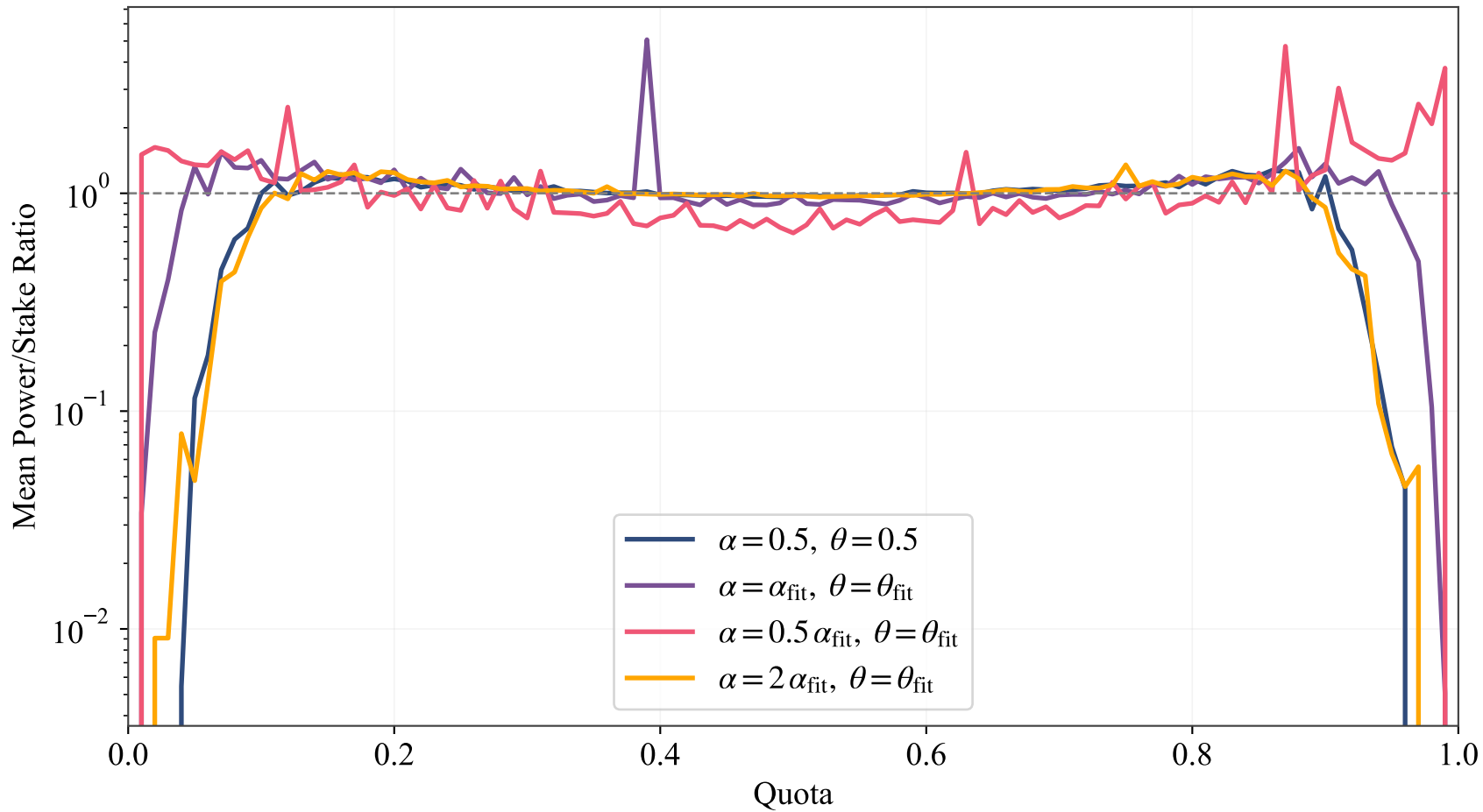
Mean Ratio vs Quota (n=50) Multiple Gamma Parameters
