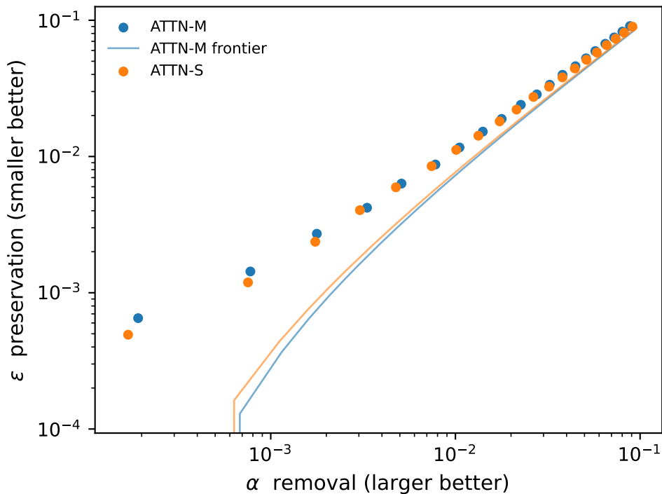
Bernoulli label flip (stochastic) — removal/preservation plane
