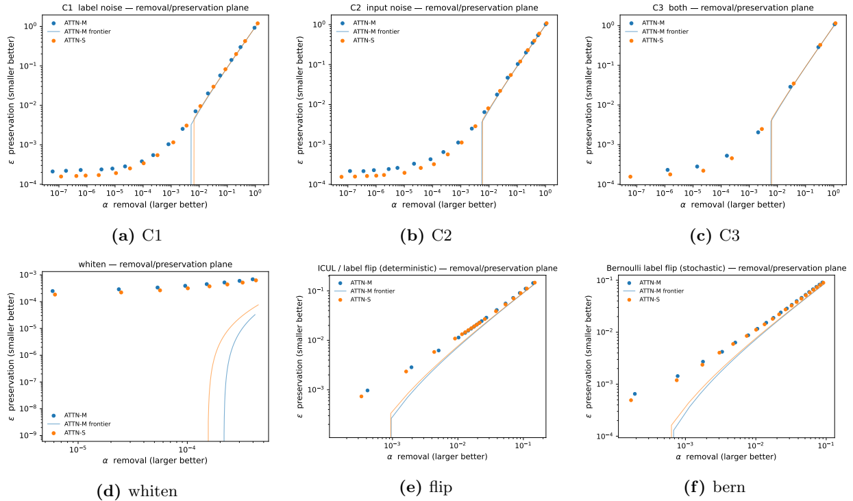
Figure 11: Frontiers, MNIST.
