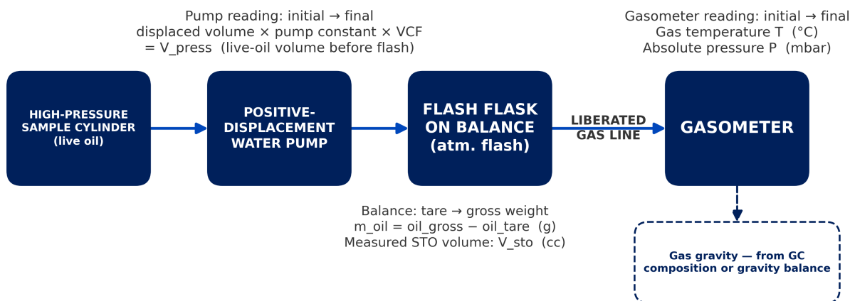
Figure 1: Atmospheric flash apparatus - displacement pump, flash line, stock-tank flask, and gasometer
