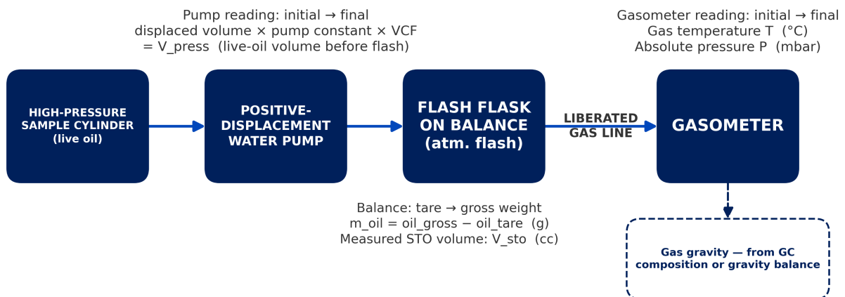
Figure 3.3 - The three instrument readings the Manual Entry form is built around: pump, stock-tank flask/balance, gasometer.
