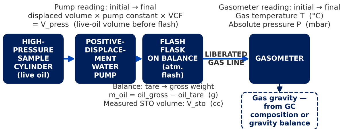
Figure 3.3 - The three instrument readings the Manual Entry form is built around: pump, stock-tank flask/balance, gasometer.
