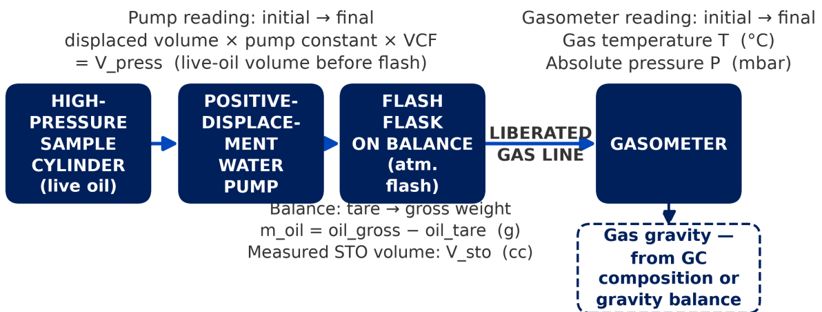
Figure 1: Atmospheric flash apparatus - displacement pump, flash line, stock-tank flask, and gasometer
