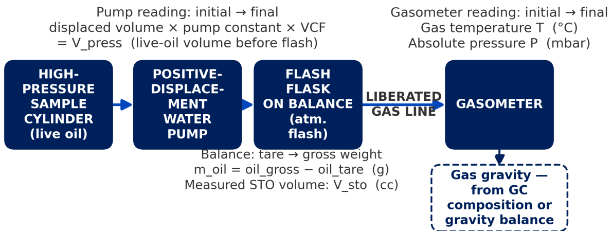
Figure 1: Atmospheric flash apparatus - displacement pump, flash line, stock-tank flask, and gasometer
