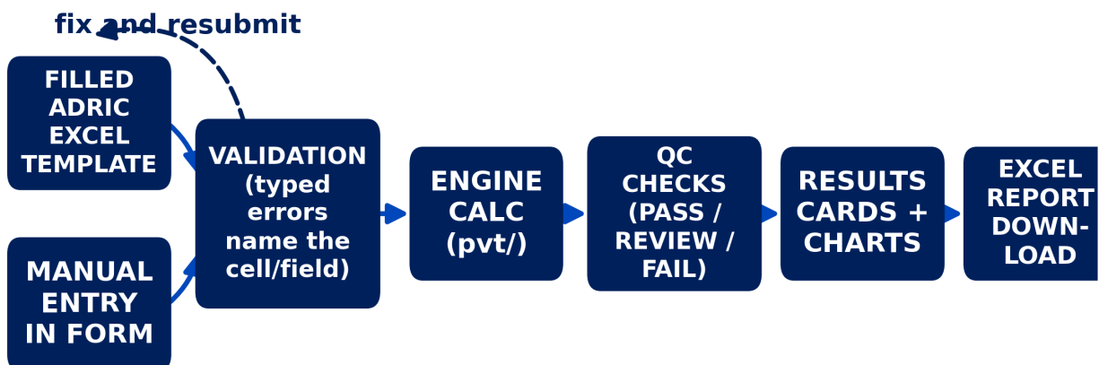
Figure 3.2 - One flow, two entry points: manual form or workbook upload, both landing on the same validated result and the same downstream rendering.
