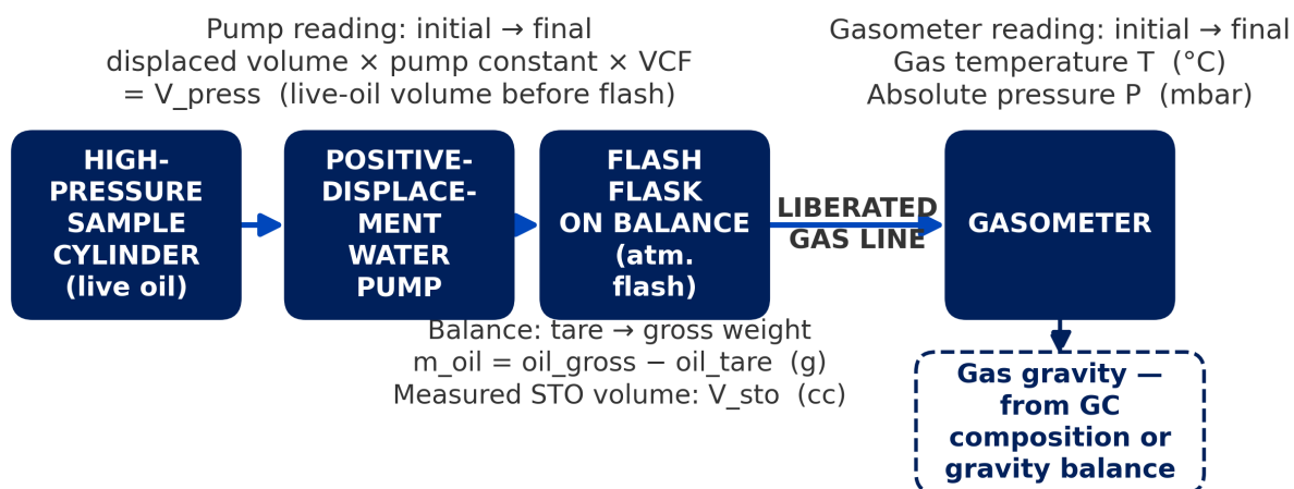
Figure 3.3 - The three instrument readings the Manual Entry form is built around: pump, stock-tank flask/balance, gasometer.
