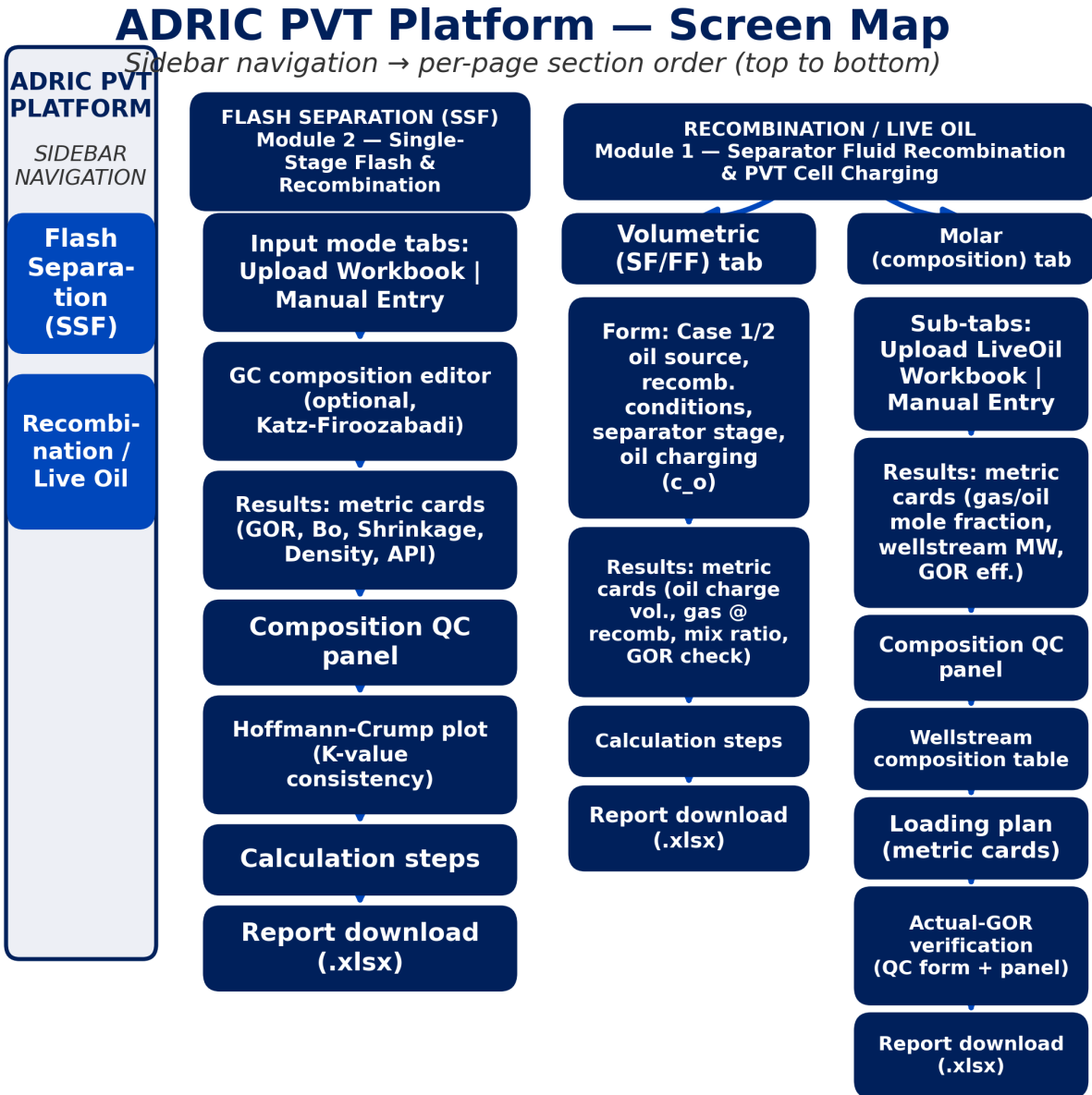
Figure 3.1 - The two pages, and the shared building blocks (page header, metric cards, QC pills, calc-steps expander, report download) every screen in the app is assembled from.
