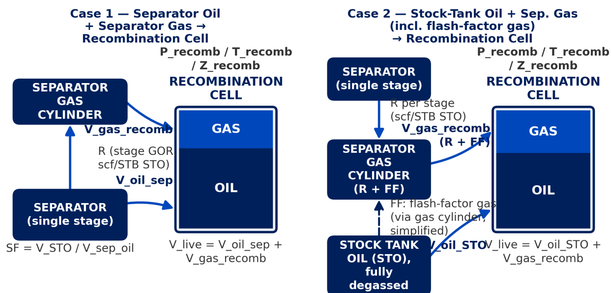
Figure 2: Recombination scheme - stock-tank oil and separator gas metered back together into a live reservoir-fluid sample
