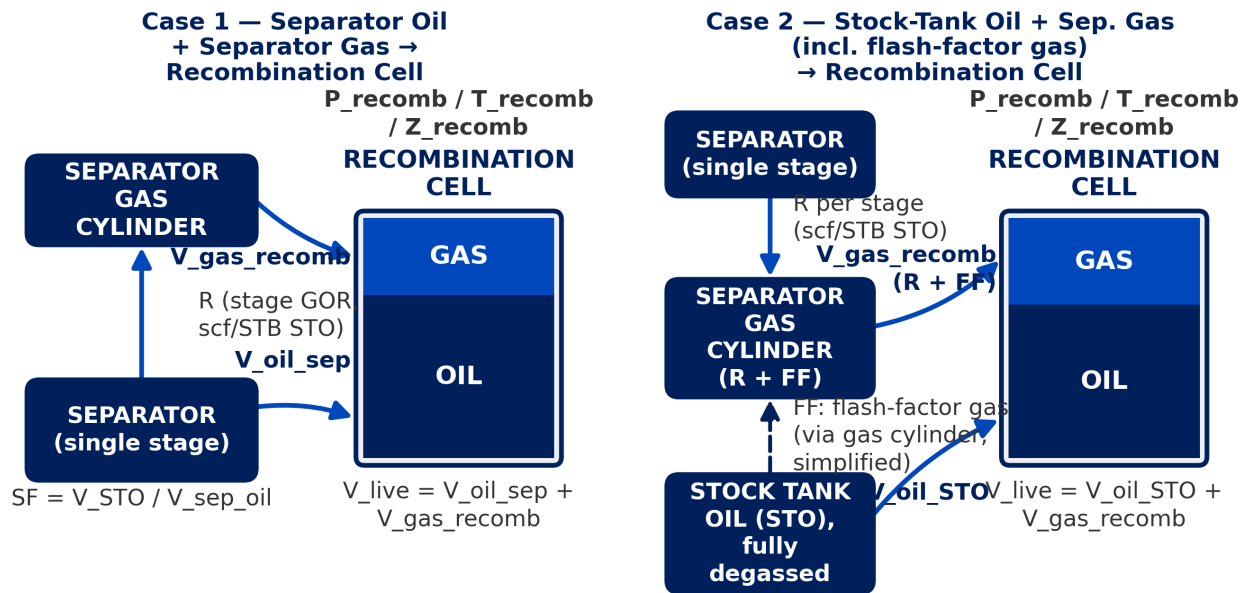
Figure 3.4 - What “recombination” means at the bench: separator (or stock-tank) oil and gas cylinder gas, metered together to reproduce the reservoir GOR.
