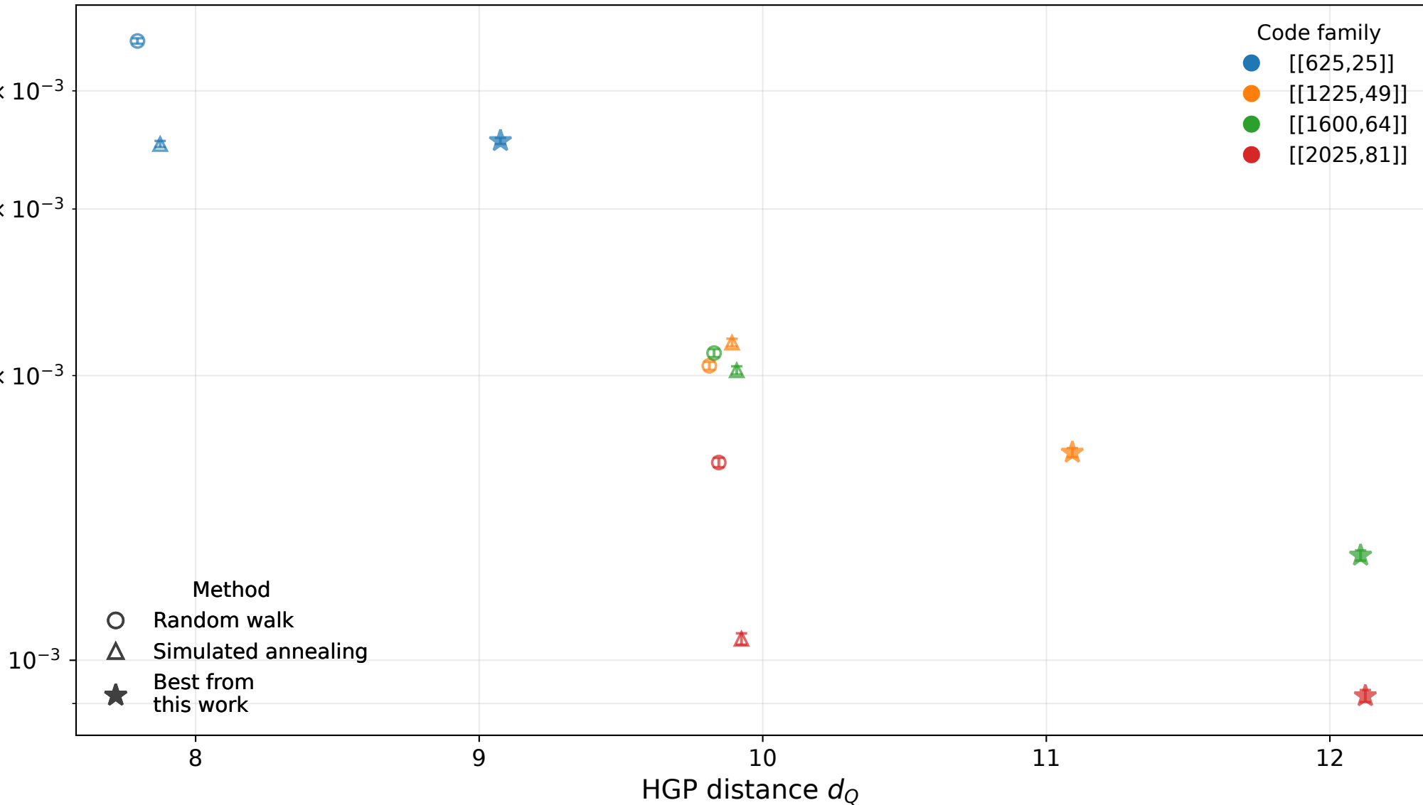
LER vs. HGP distance for optimized HGP codes
