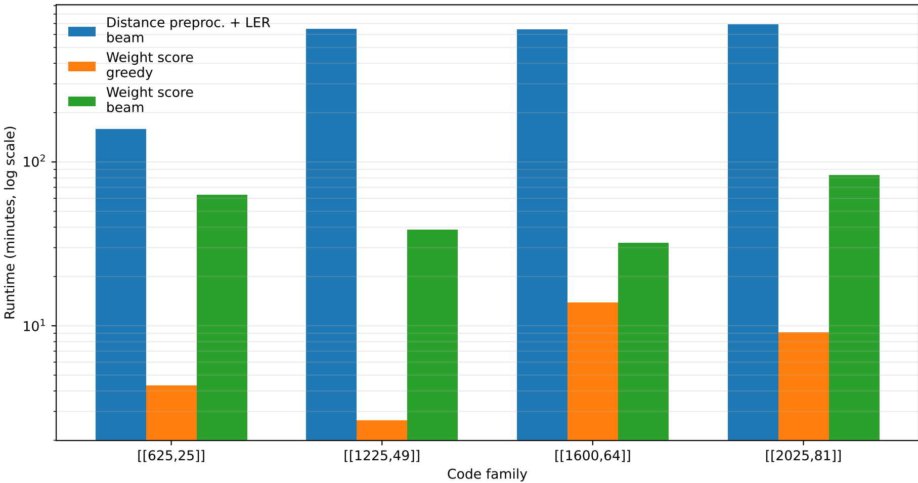
Runtime comparison of optimization methods
