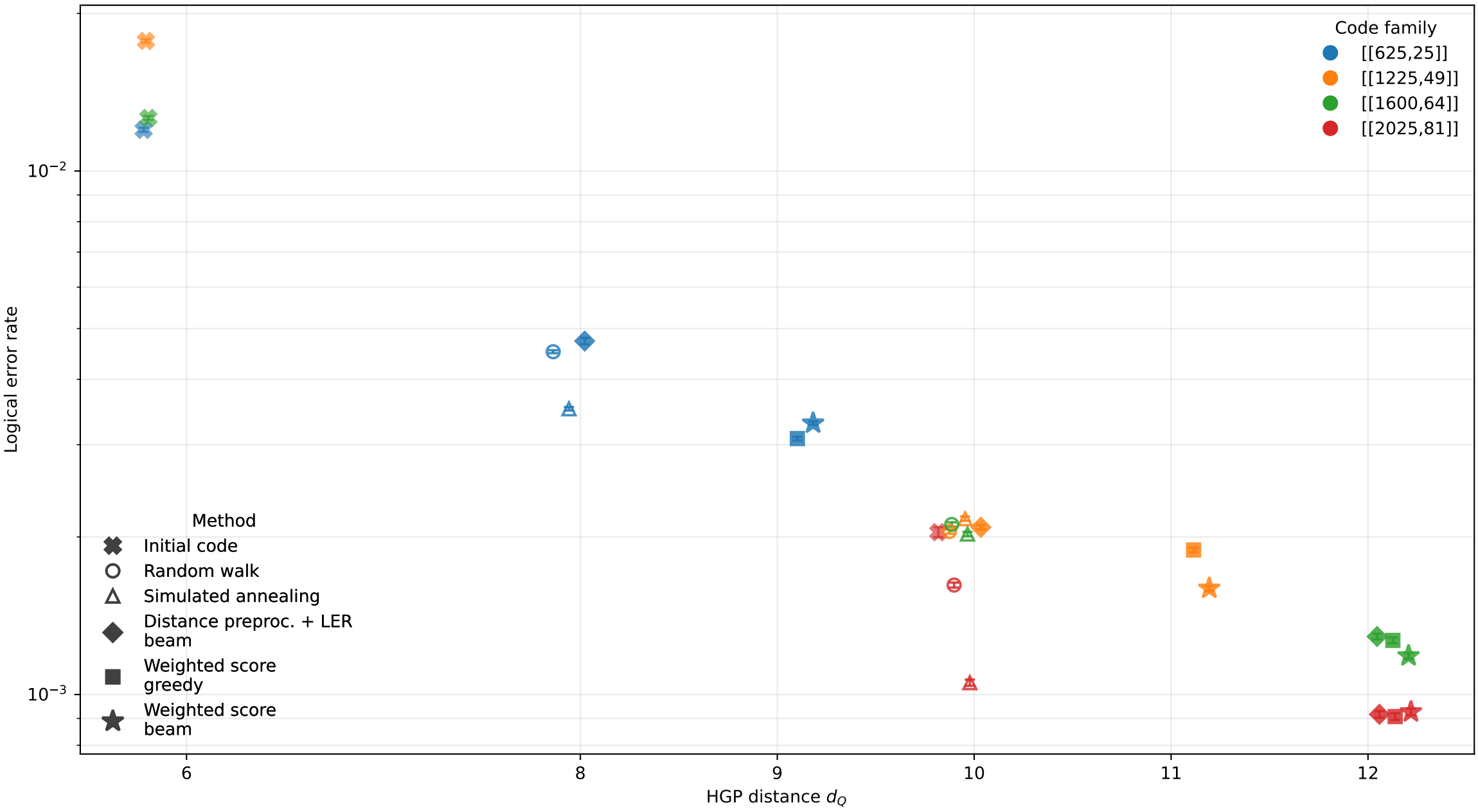
Distance and logical error rate of initial and optimized HGP codes
