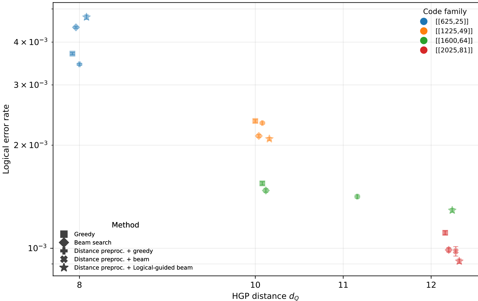
LER vs. HGP distance for optimized HGP codes
