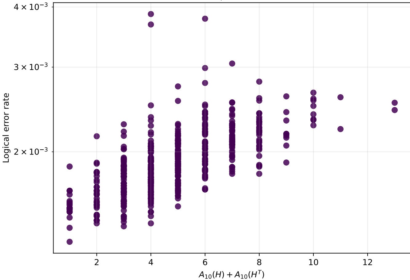
LER vs. A_{d_Q} ( d_Q = 10 only)
