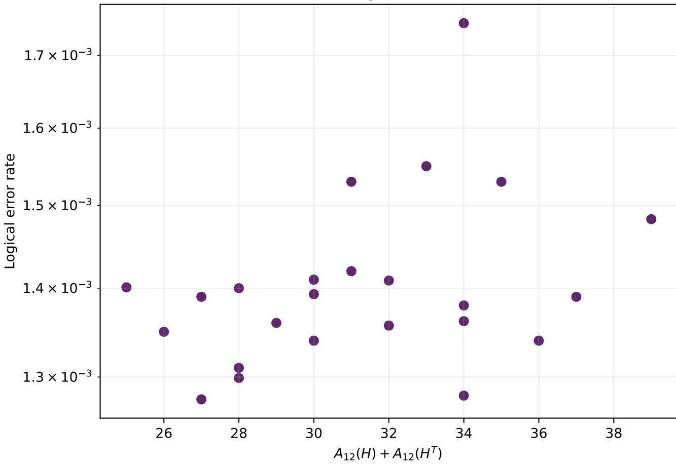
LER vs. A_{d_Q} ( d_Q = 12 only)
