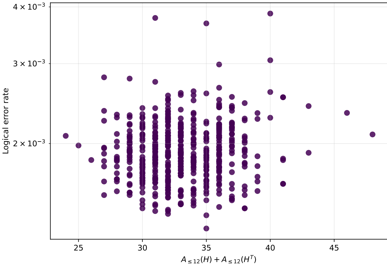
LER vs. low-weight undetectable patterns ( d_Q = 10 only)
