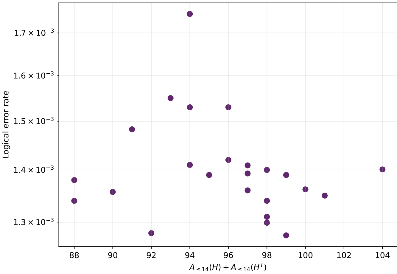
LER vs. low-weight undetectable patterns ( d_Q = 12 only)
