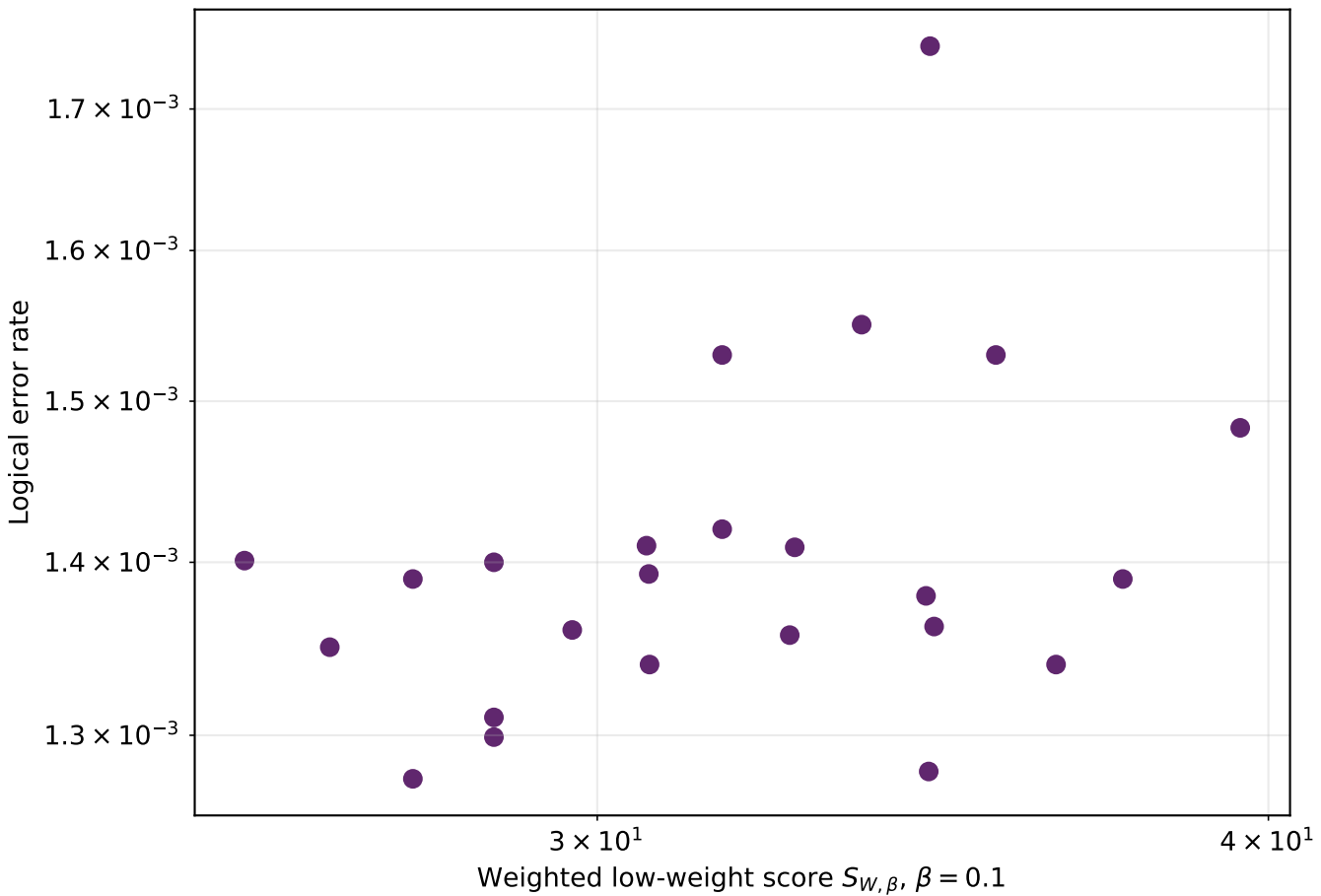
LER vs. weighted score, \beta = 0.1 ( d_Q = 12 only)
